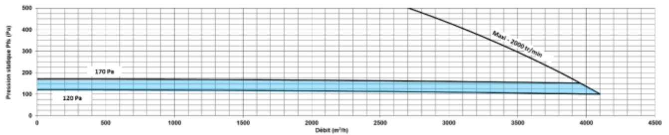
Figure 43 - ECOBLUE® 2600 (monophasé)
