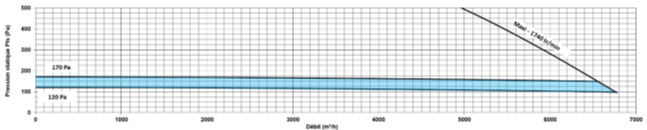
Figure 44 - ECOBLUE® 4200 (monophasé)
