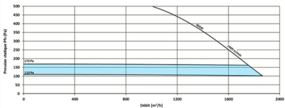
Figure 41 - ECOBLUE® 1000 (monophasé)
