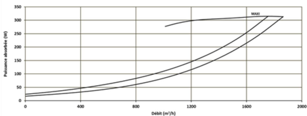
Figure 42 - ECOBLUE® 1800 (monophasé)
