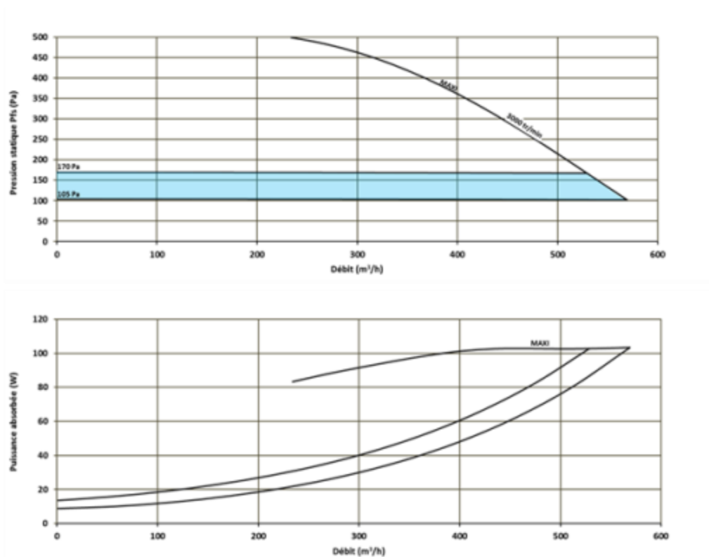
Figure 40 - ECOBLUE® 600 (monophasé)
