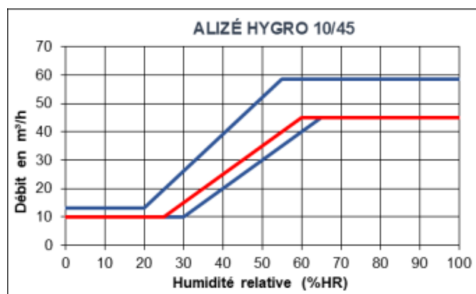
Figure 26 – HB03 – ALIZÉ HYGRO 10-45 (25-60%HR)
