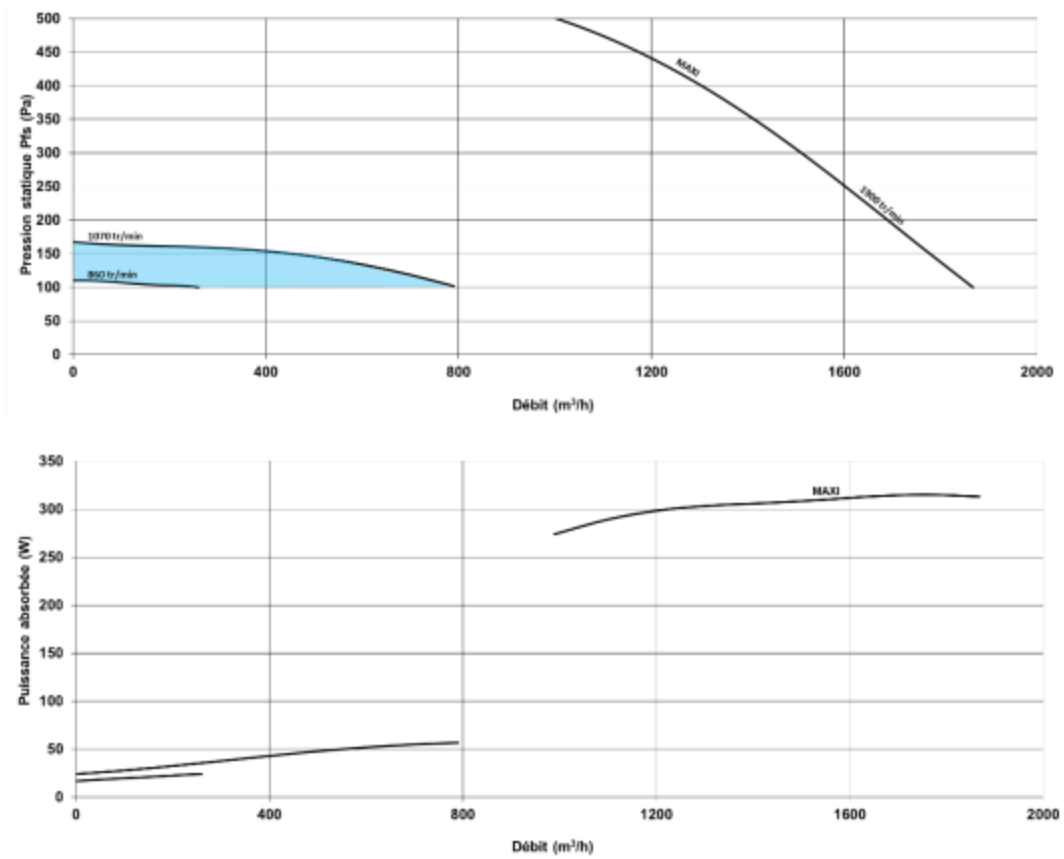
Figure 56 - ECOBLUE® 1800 ECONIZER (OU ECONIZER 1800)
