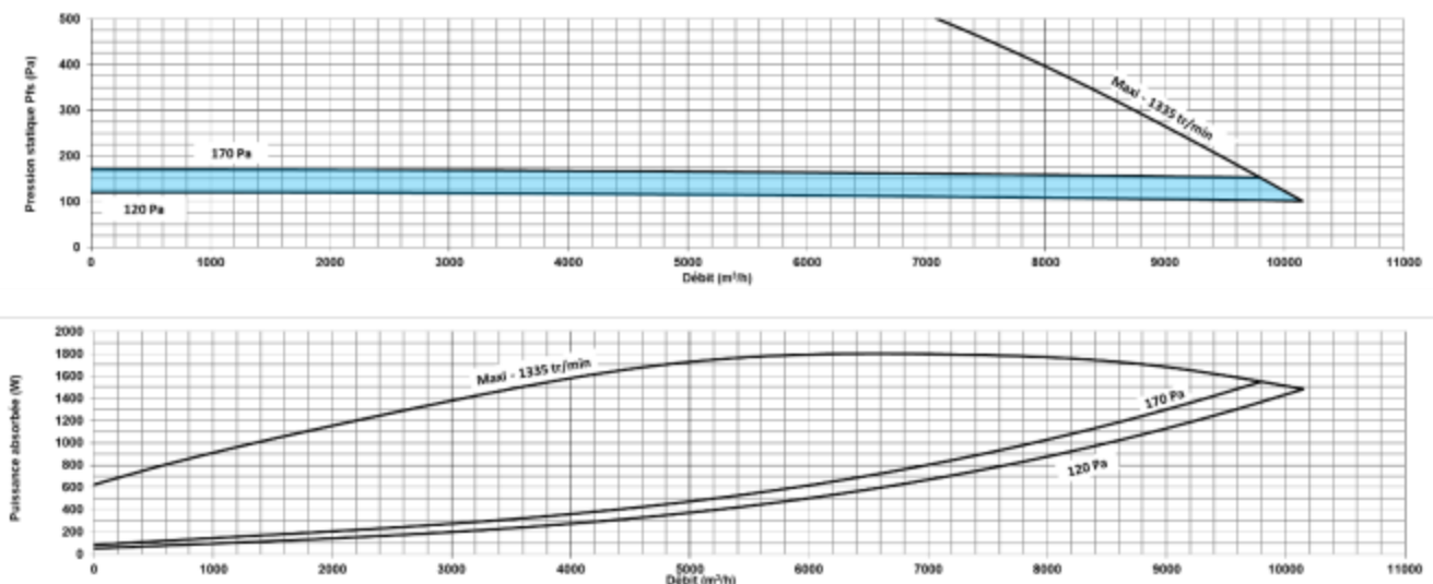
Figure 47 - ECOBLUE® 11000 (triphasé)
