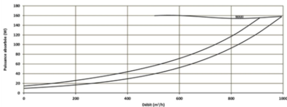
Figure 41 - ECOBLUE® 1000 (monophasé)
