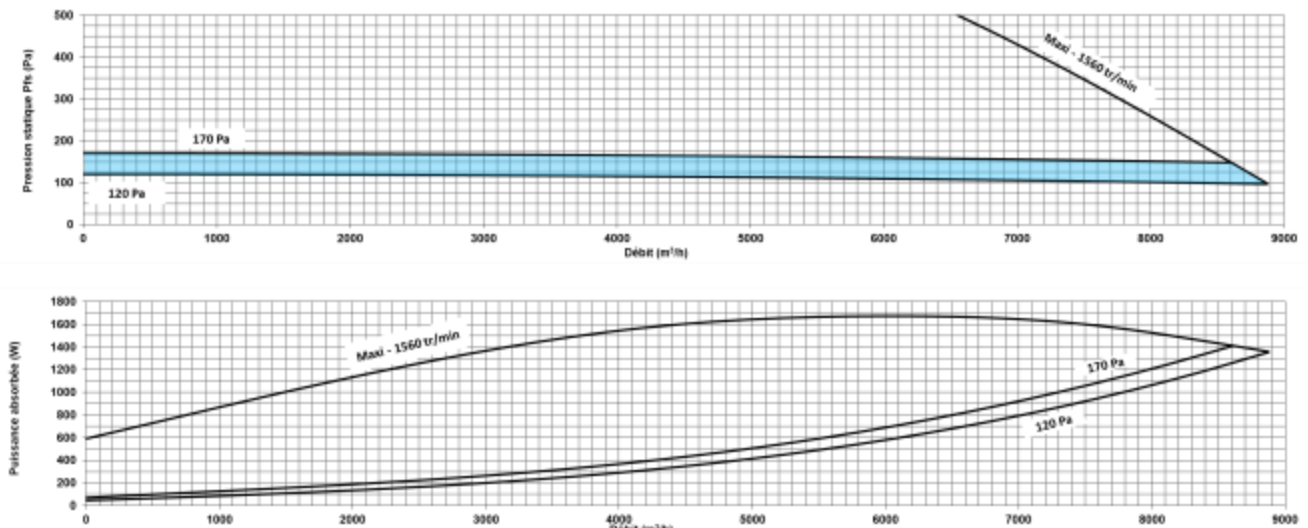
Figure 46 - ECOBLUE® 9100 (triphasé)
